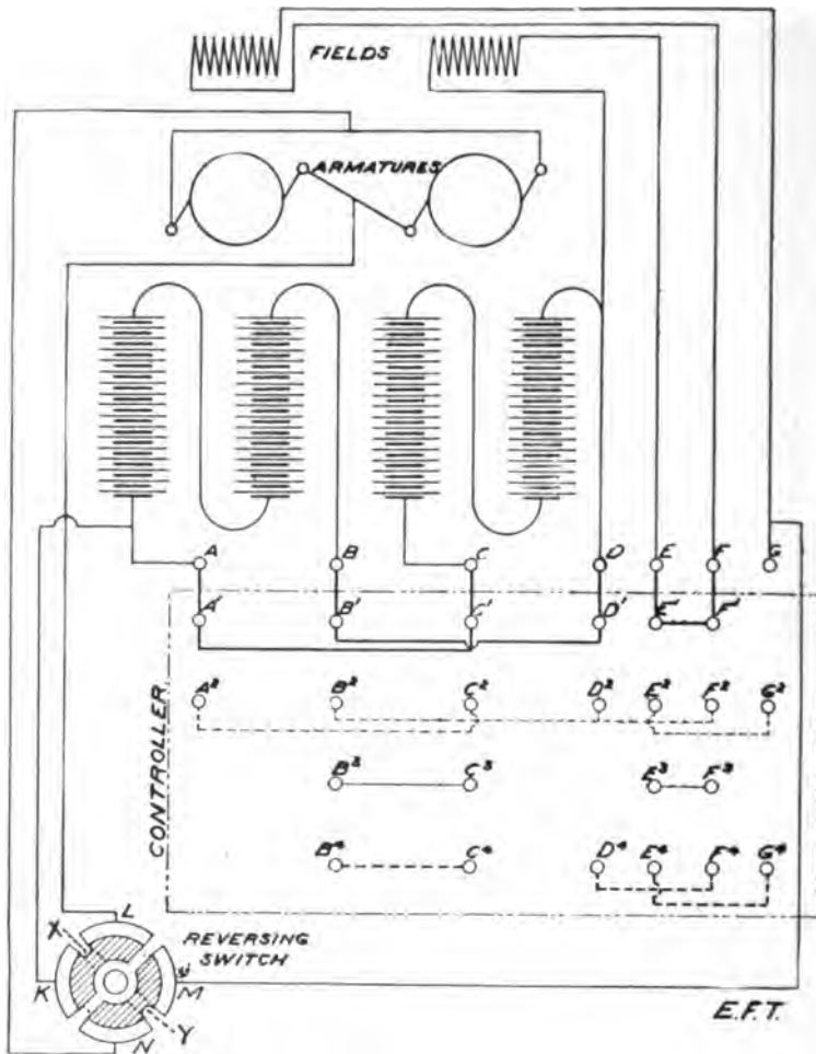
FIG. 441. —Diagram Plan of the Several Parts of an Electrical Vehicle Driving Circuit. The field-windings and armatures are shown projected, the proper wiring connections being indicated. The periphery of the controller is laid out within the broken line rectangle, the contacts and connections through it for varying the circuits through four speeds being shown. A, B, C, D, E, F, G are the terminal contact points of the various speed circuits, to be made as the positions of the controller contacts are varied. A', B', C', D', E', F' are the controller contacts, which, with those already mentioned, make the proper circuits for the first speed. Similarly, A'', B'', C'', etc., when brought into contact with A, B, C, etc., give the second speed circuits; B'', C'', D'', E'', F'', G'', in contact with A, B, C, D, etc., give the third speed; and B''', C''', D''', in the same manner, the fourth speed. The reverse switch gives the backward movement, as described.
